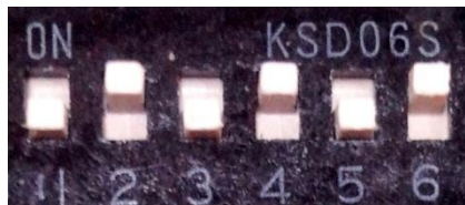
RS422 mode
